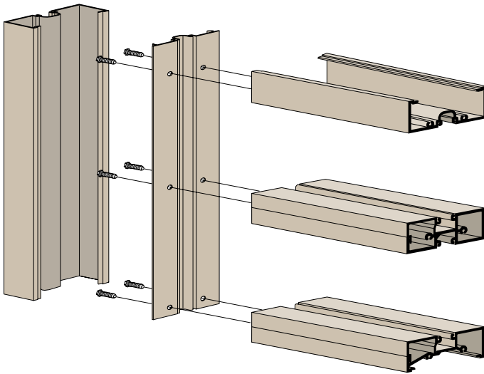
STACK ASSEMBLY
