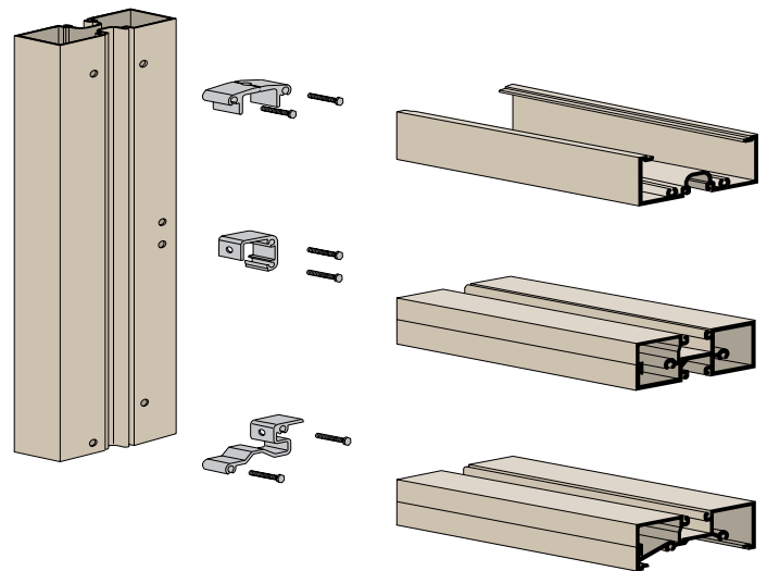
135° CORNER
