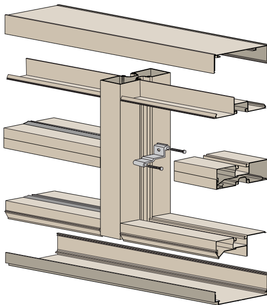
STACK ASSEMBLY
